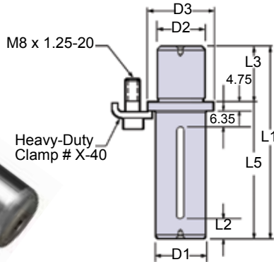
BALL-BEARING GUIDE POSTS – METRIC – Tap Fit
